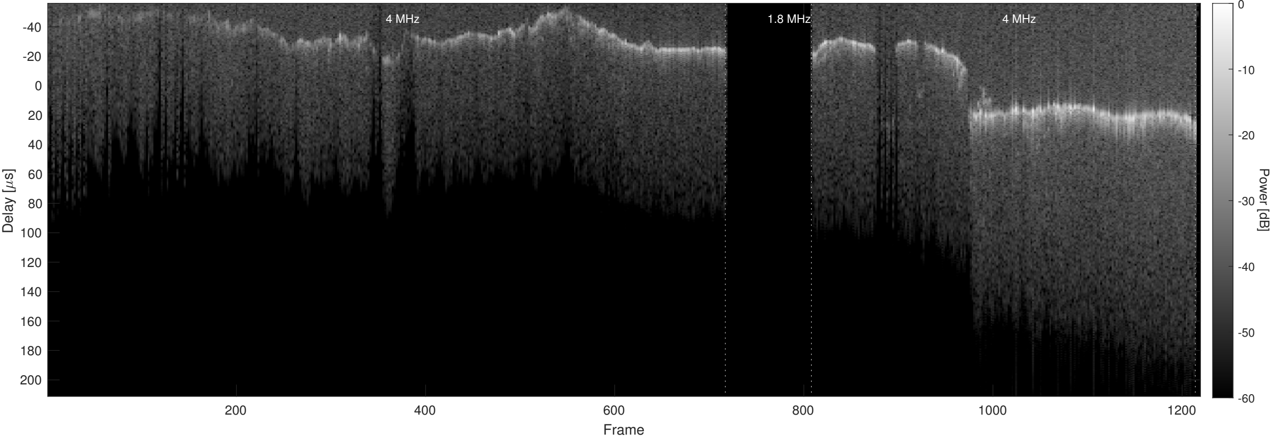
Orbit 23063, Chapman, No Window, Channel 2
