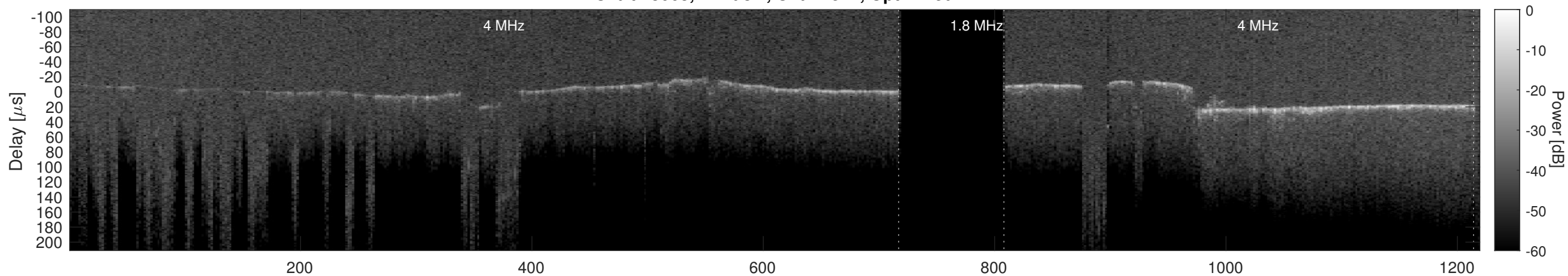
Orbit 23063, Cluttergram
