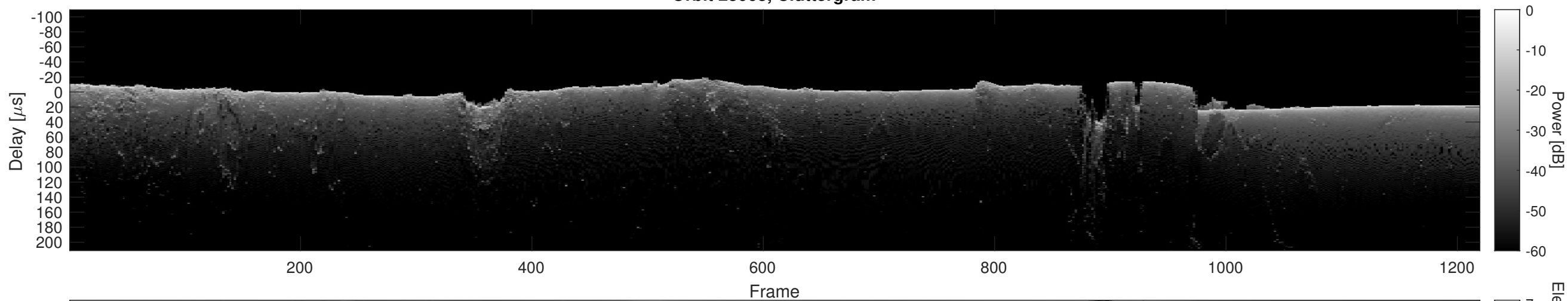
Orbit 23063, Cluttergram
