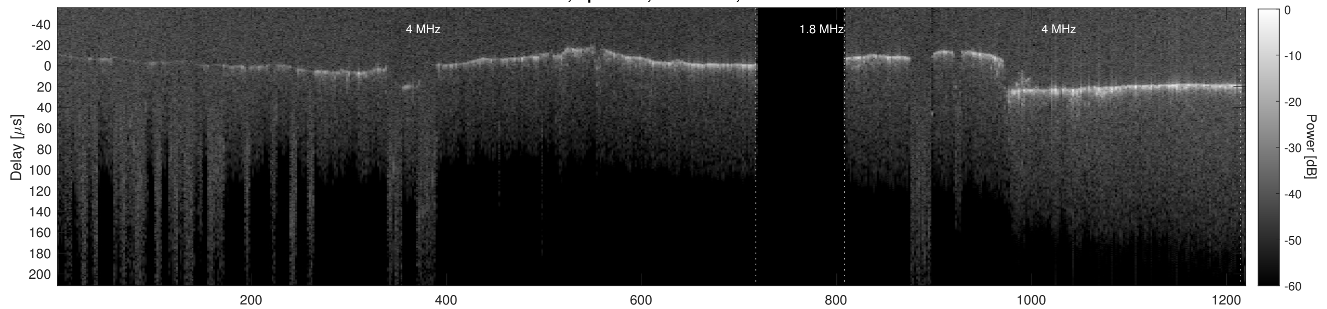
Orbit 23063, Cluttergram
