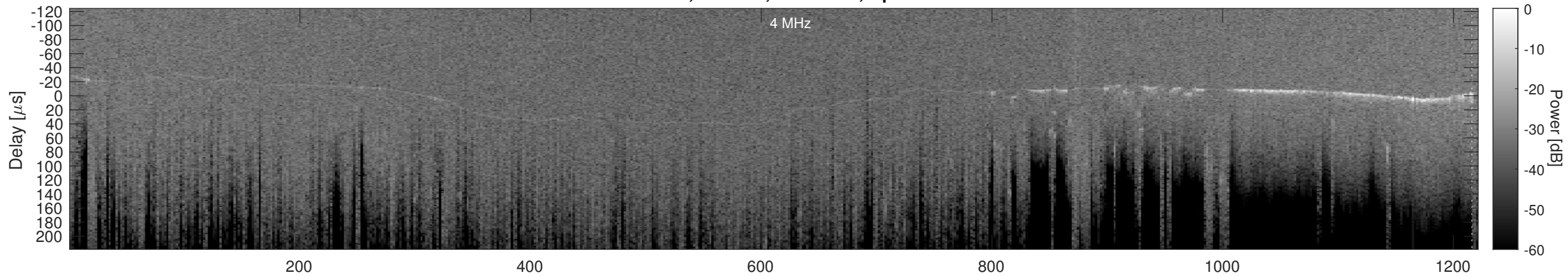
Orbit 23065, Cluttergram
