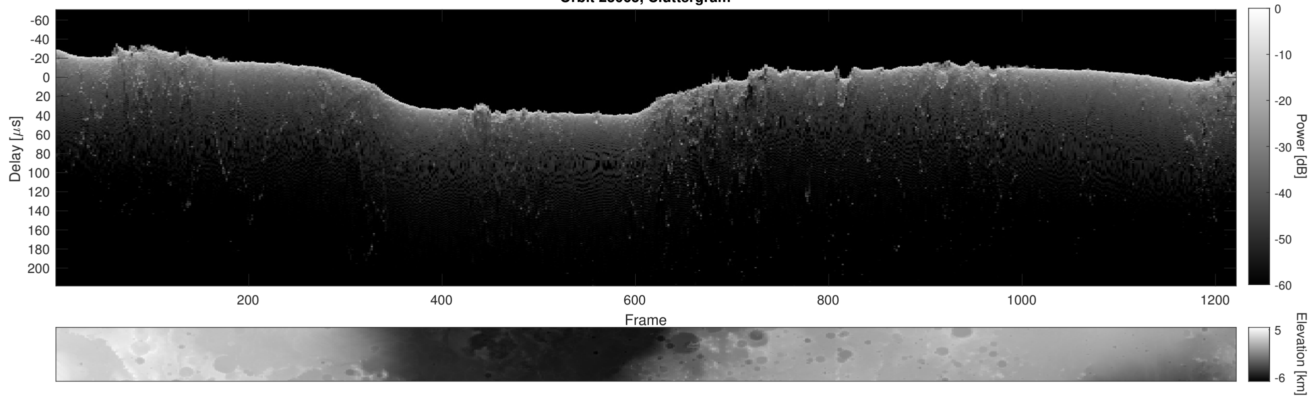
Orbit 23065, Cluttergram
