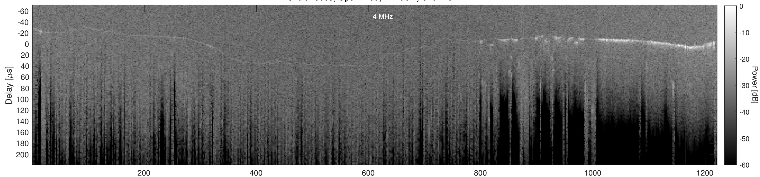
Orbit 23065, Cluttergram
