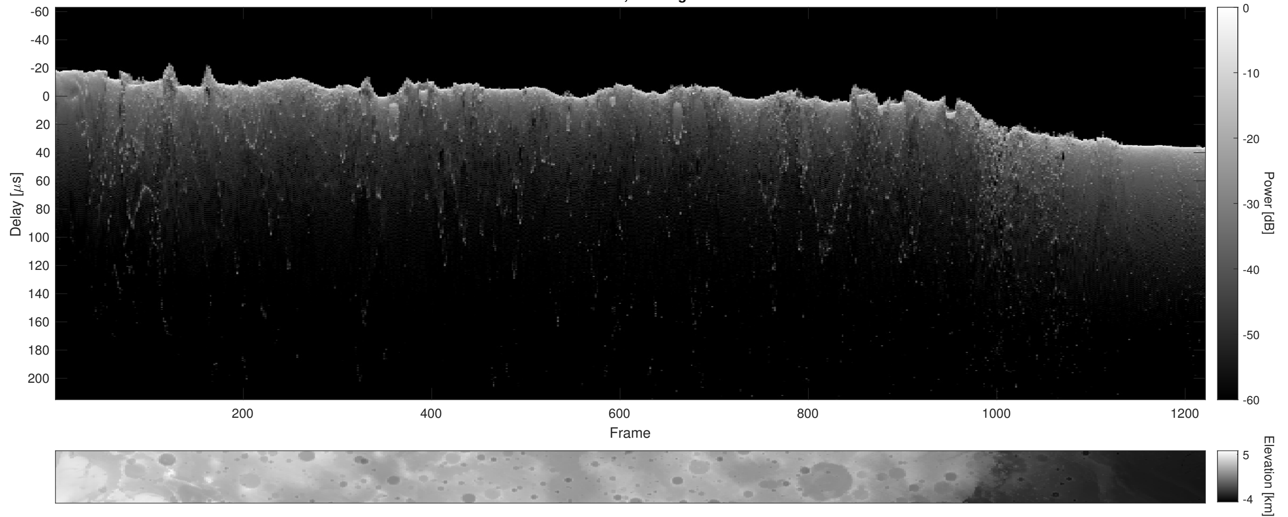
Orbit 23068, Cluttergram
