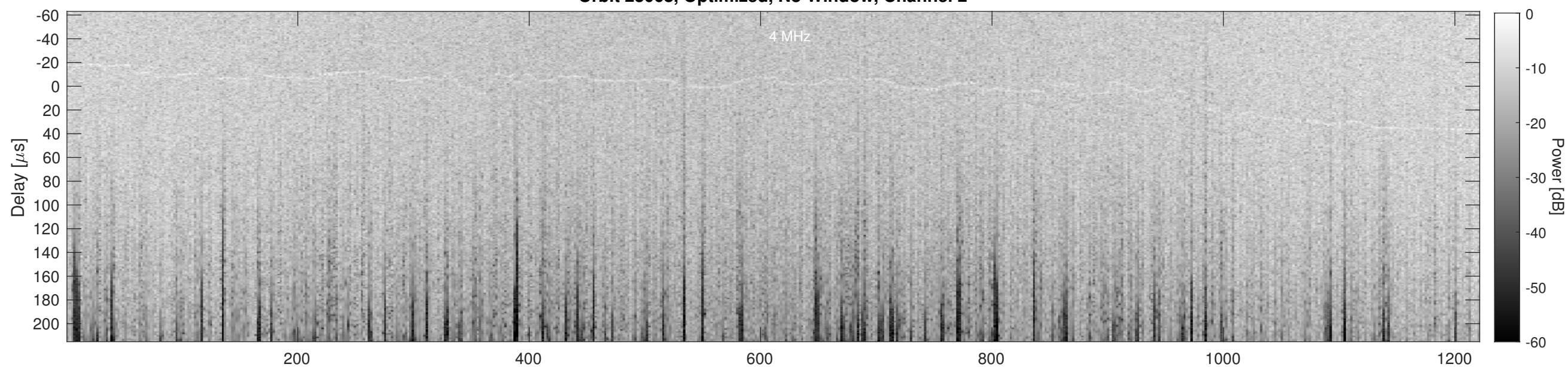
Orbit 23068, Cluttergram
