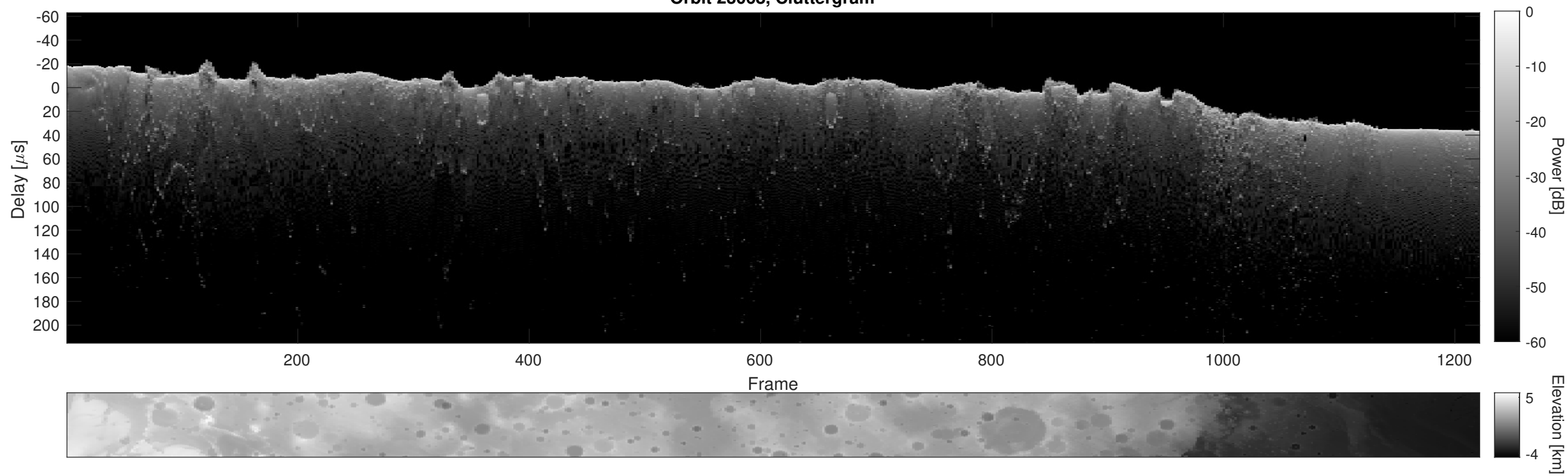
Orbit 23068, Cluttergram
