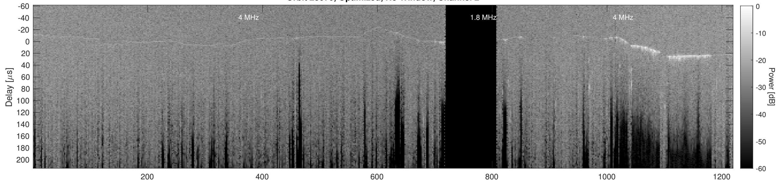
Orbit 23070, Cluttergram
