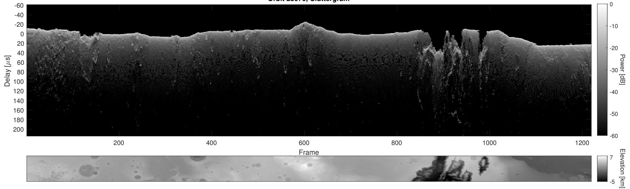
Orbit 23070, Cluttergram
