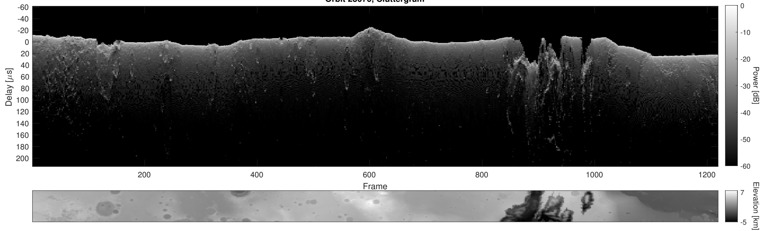
Orbit 23070, Cluttergram
