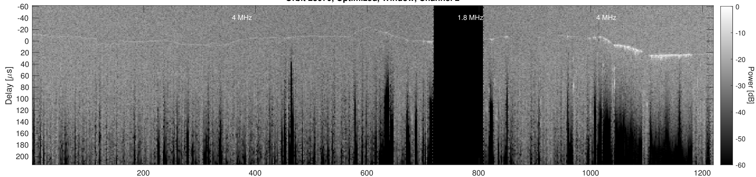
Orbit 23070, Cluttergram
