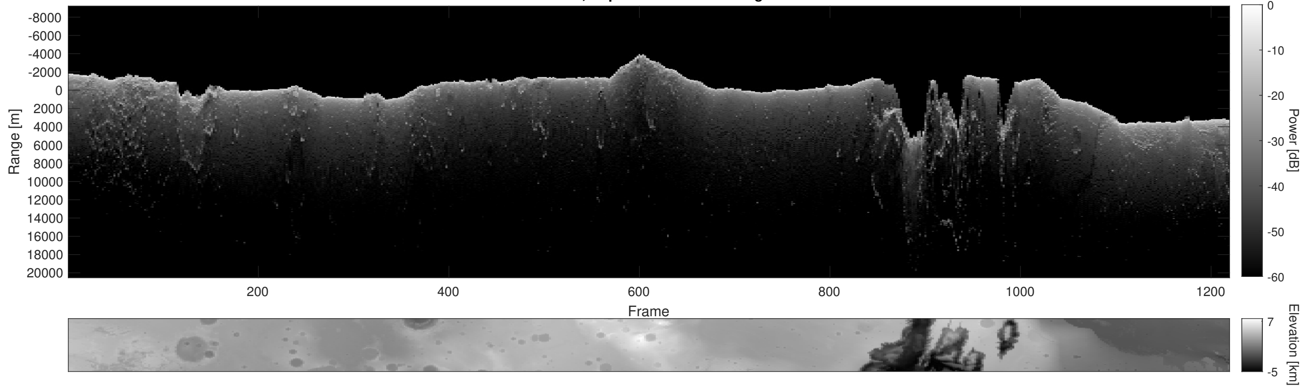
Orbit 23070, Depth-Corrected Cluttergram
