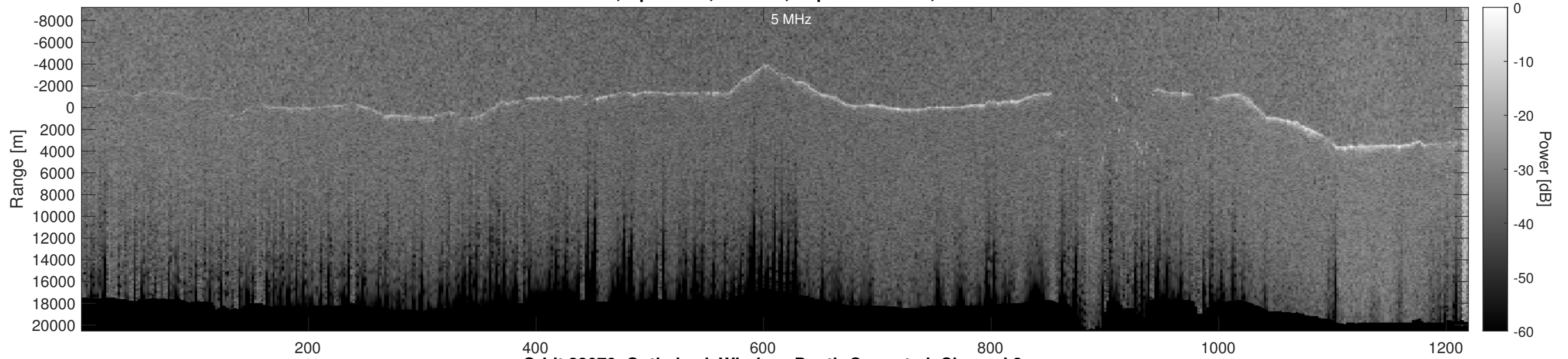
Orbit 23070, Optimized, Window, Depth-Corrected, Channel 2
