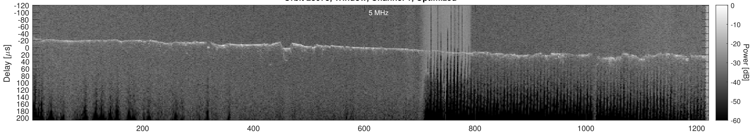
Orbit 23073, Cluttergram
