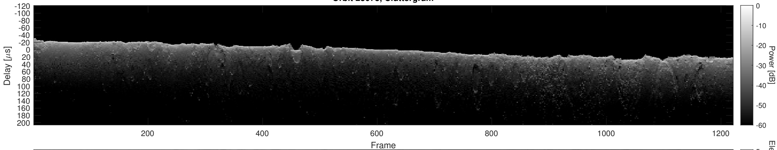
Orbit 23073, Cluttergram
