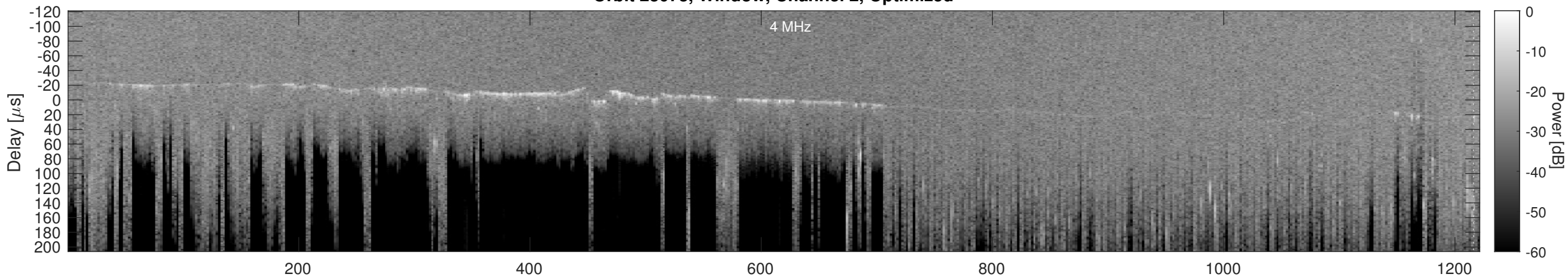
Orbit 23073, Cluttergram
