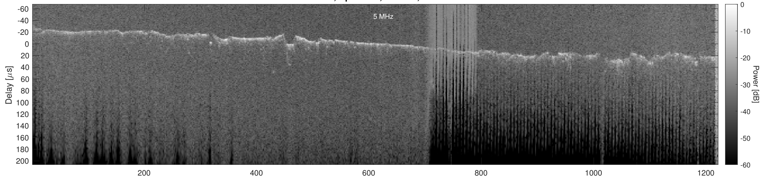
Orbit 23073, Optimized, Window, Channel 2
