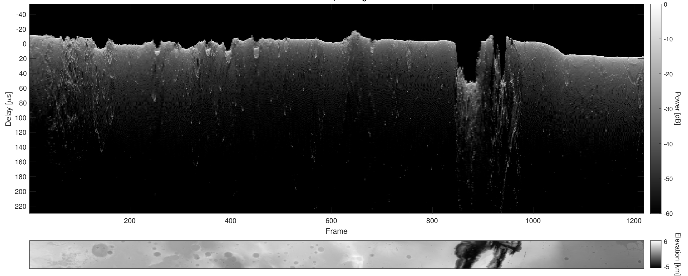
Orbit 23077, Cluttergram
