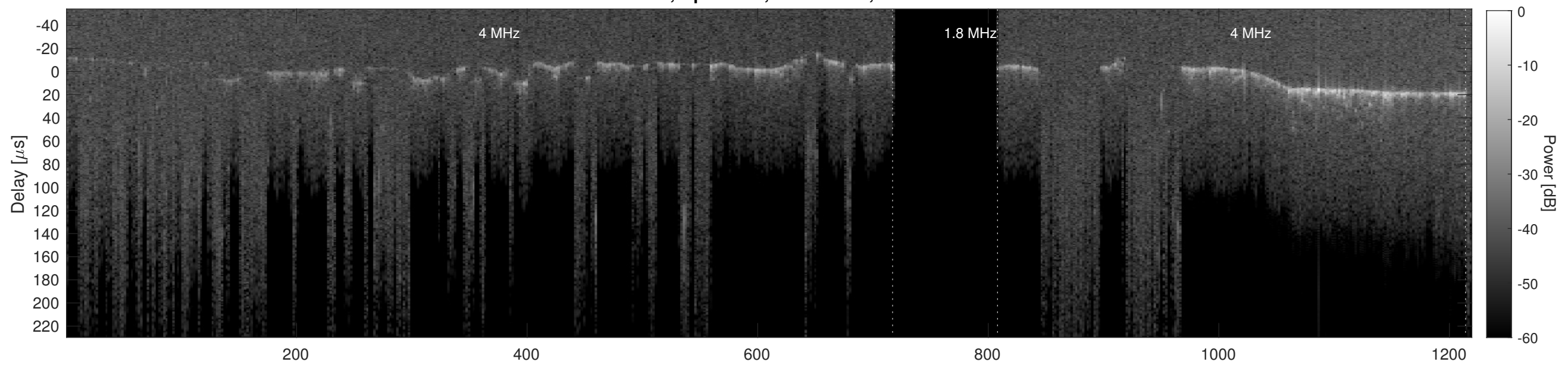
Orbit 23077, Cluttergram
