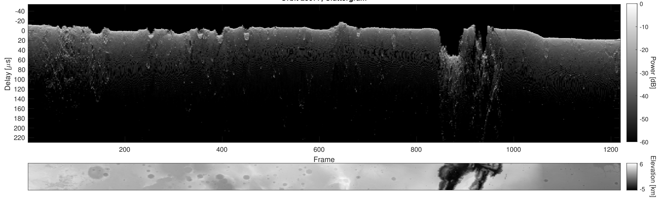
Orbit 23077, Cluttergram
