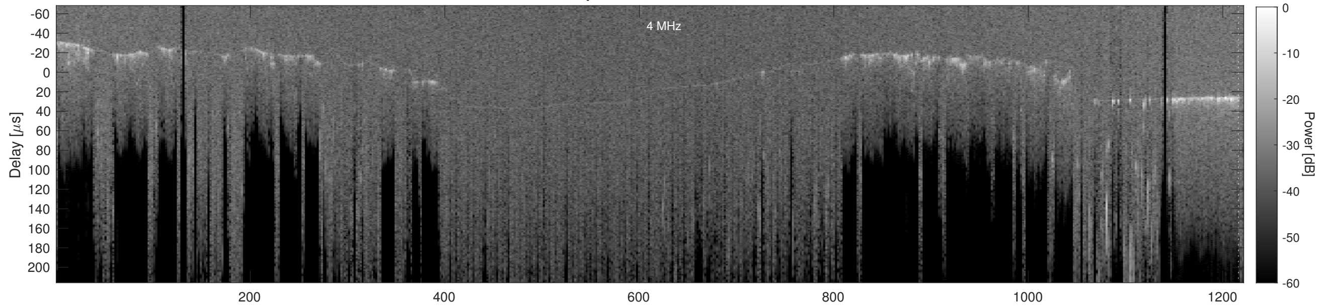
Orbit 23079, Cluttergram
