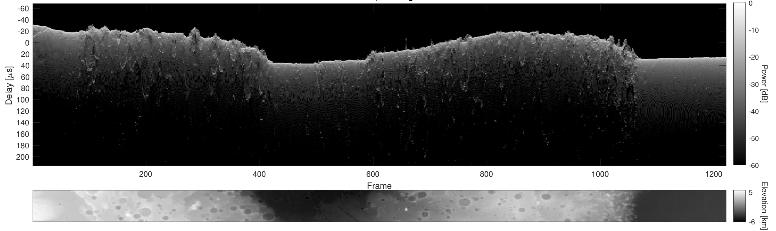
Orbit 23079, Cluttergram
