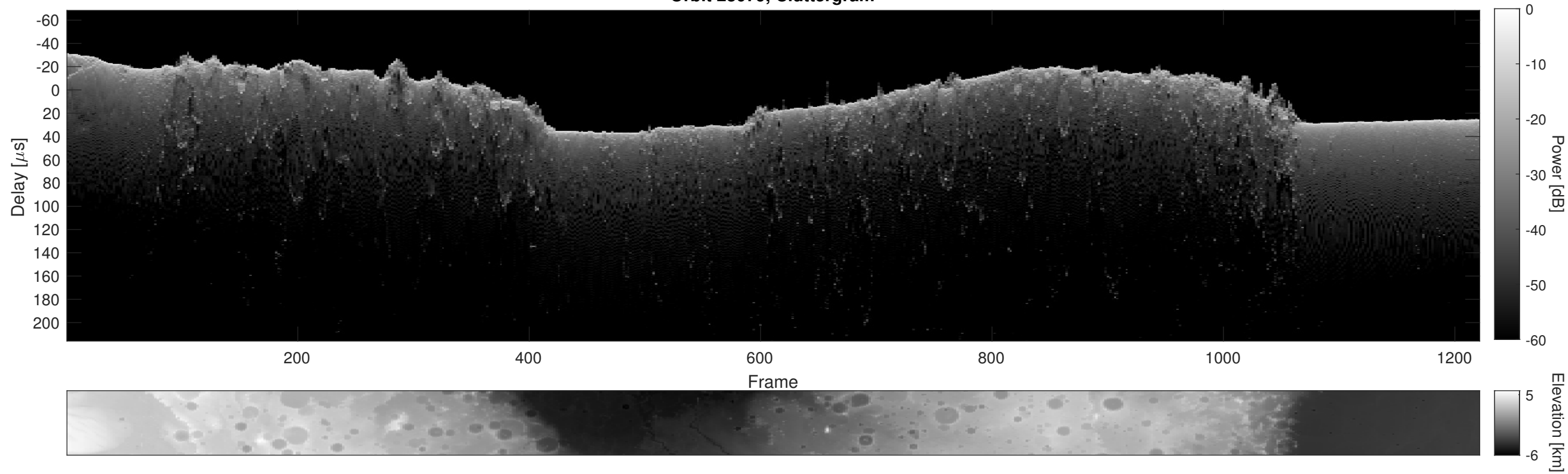
Orbit 23079, Cluttergram
