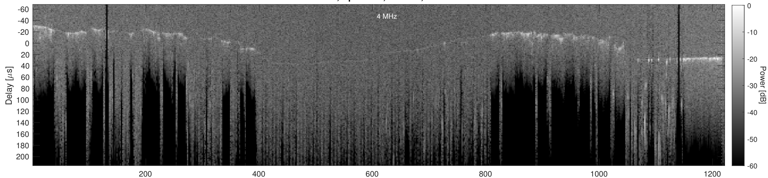
Orbit 23079, Cluttergram
