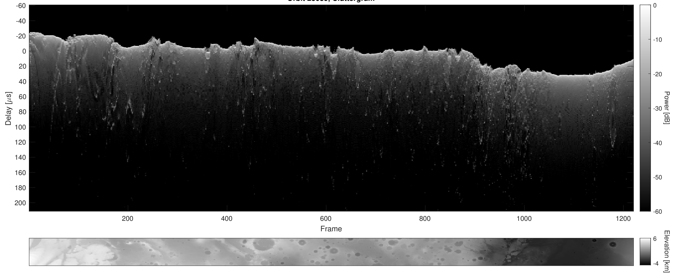
Orbit 23089, Cluttergram
