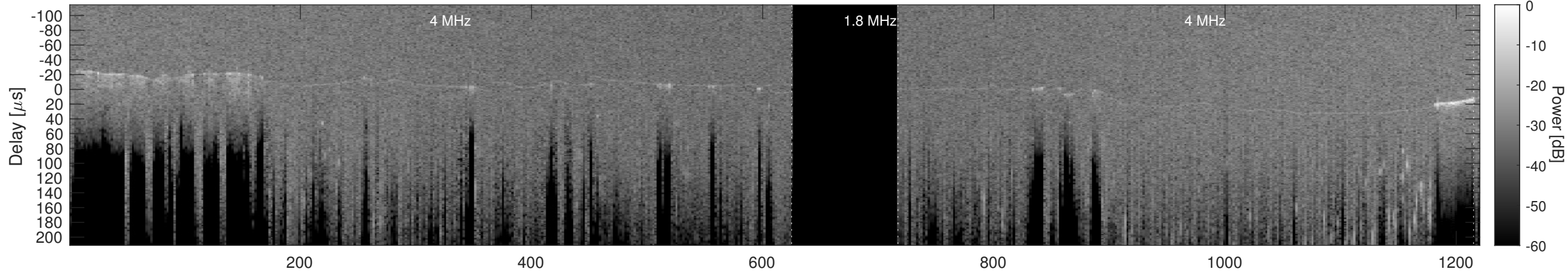
Orbit 23089, Cluttergram
