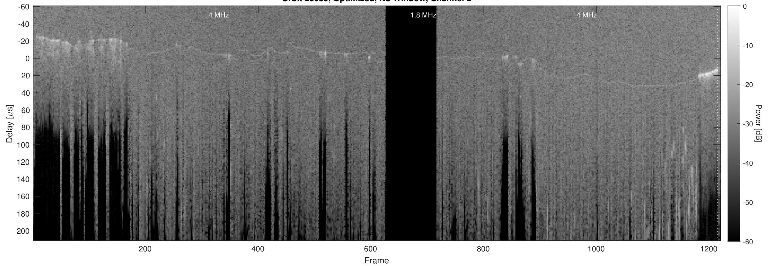
Orbit 23089, Optimized, No Window, Channel 2
