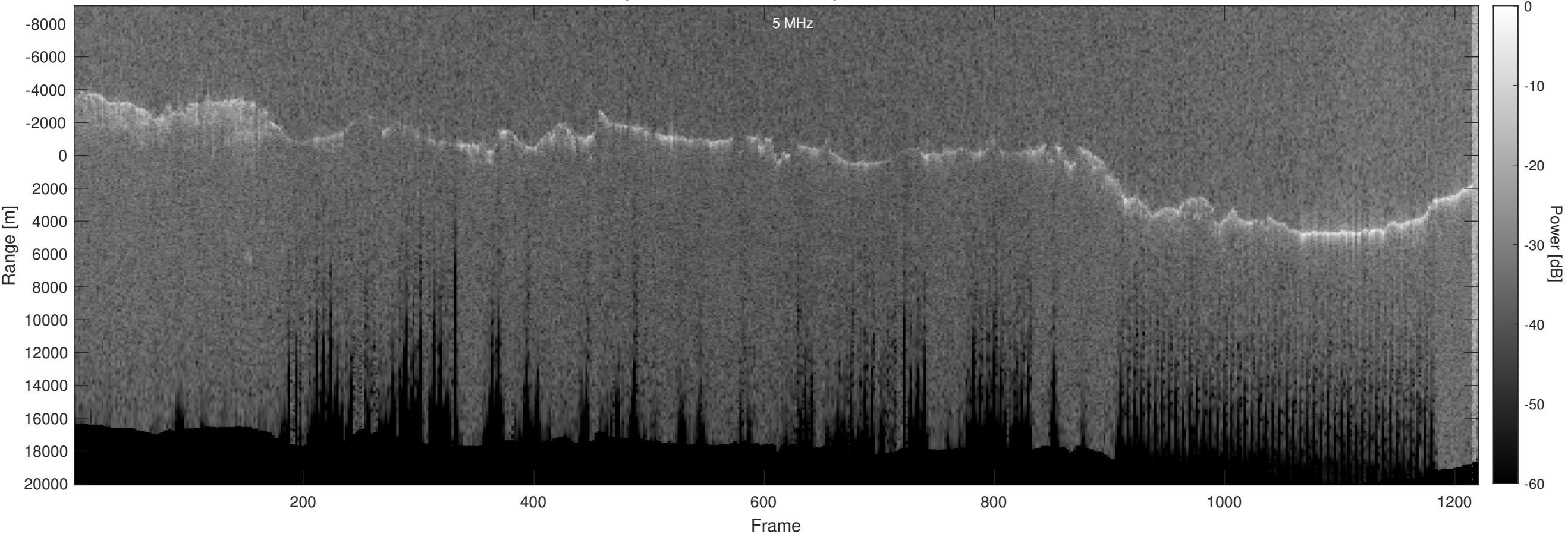
Orbit 23089, Optimized, No Window, Depth-Corrected, Channel 2
