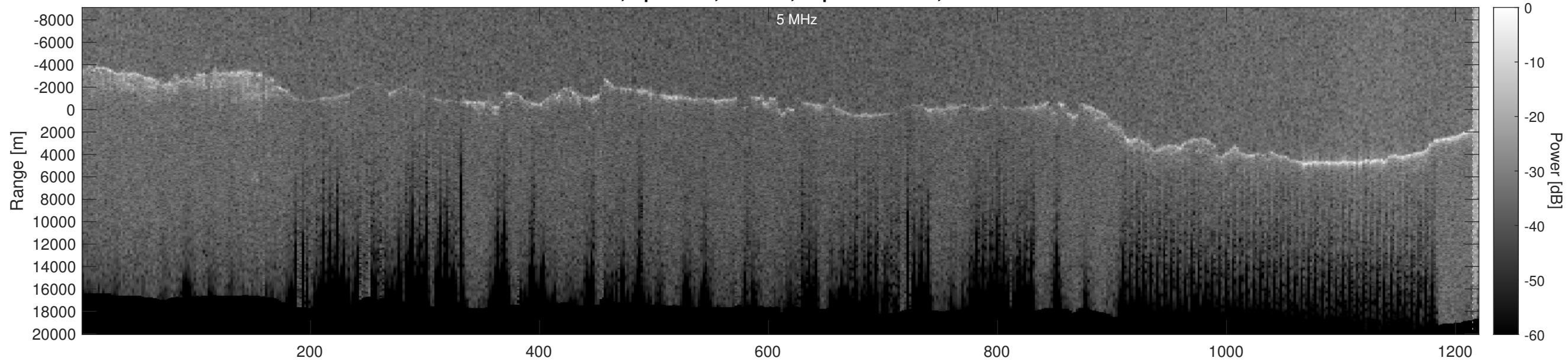
Orbit 23089, Optimized, Window, Depth-Corrected, Channel 2
