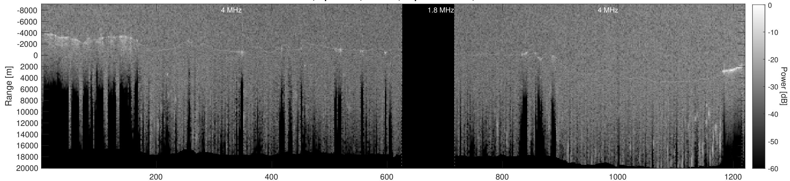
Orbit 23089, Depth-Corrected Cluttergram
