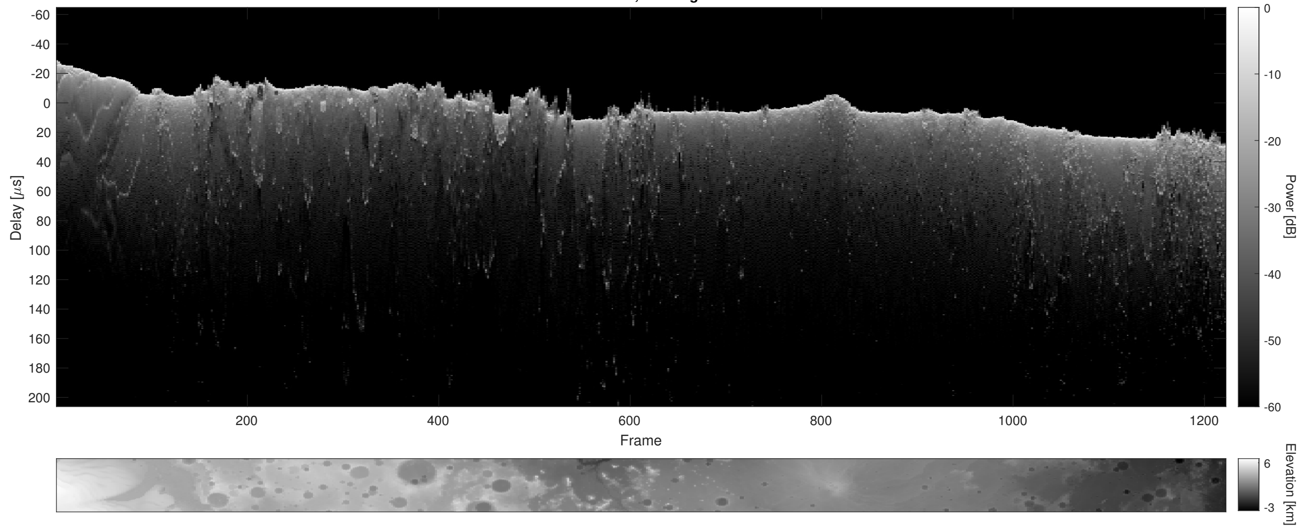
Orbit 23107, Cluttergram
