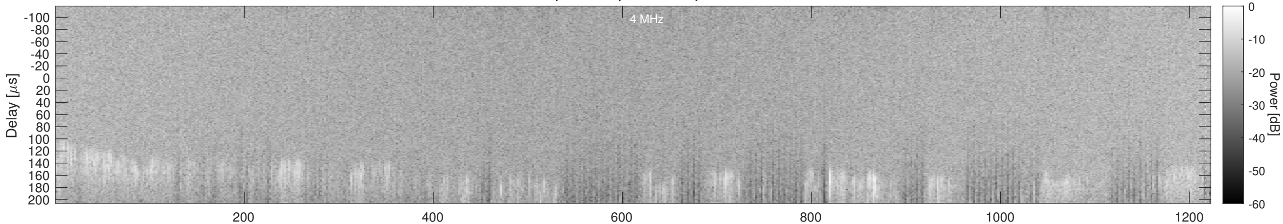
Orbit 23107, Window, Channel 2, Chapman
