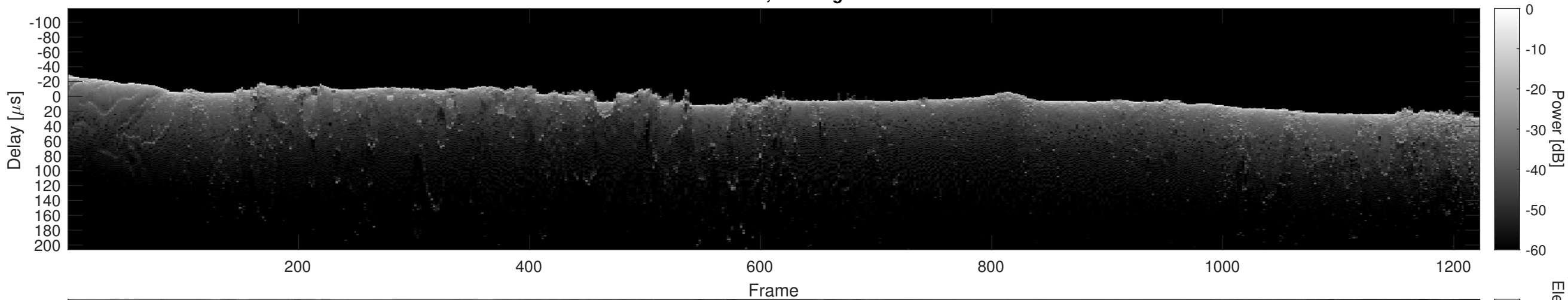
Orbit 23107, Cluttergram
