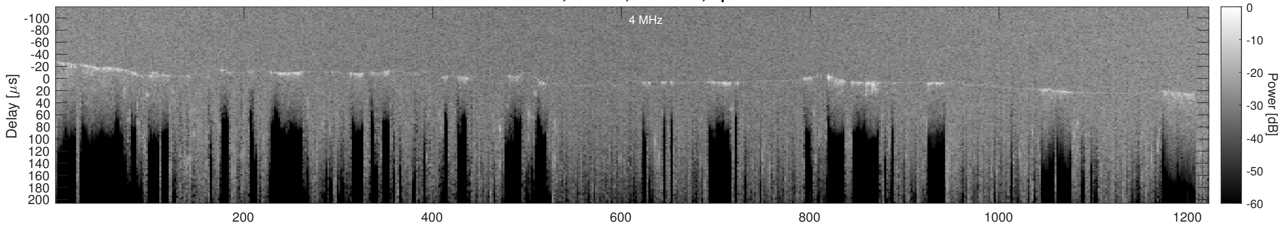
Orbit 23107, Cluttergram
