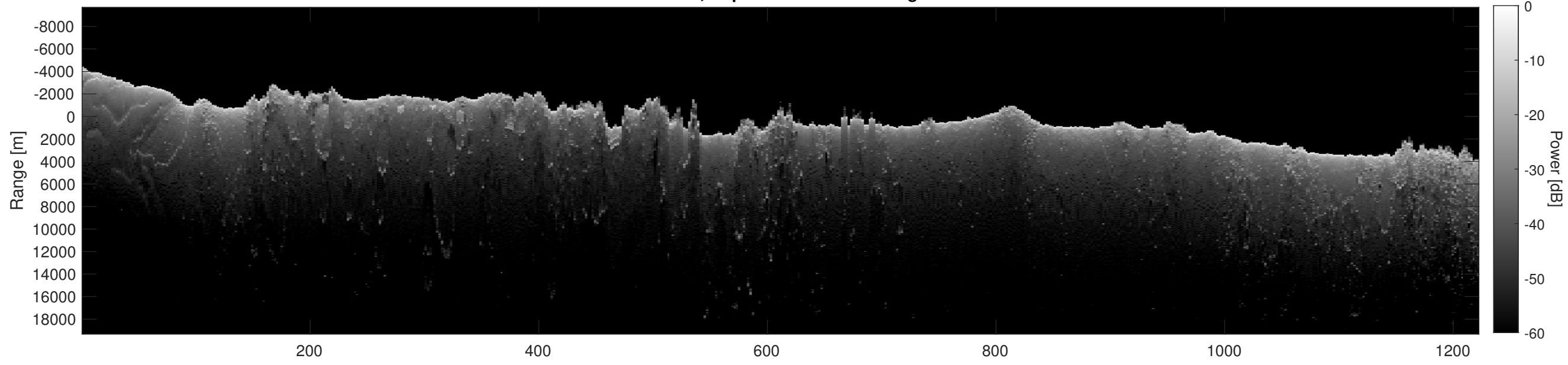
Orbit 23107, Depth-Corrected Cluttergram
