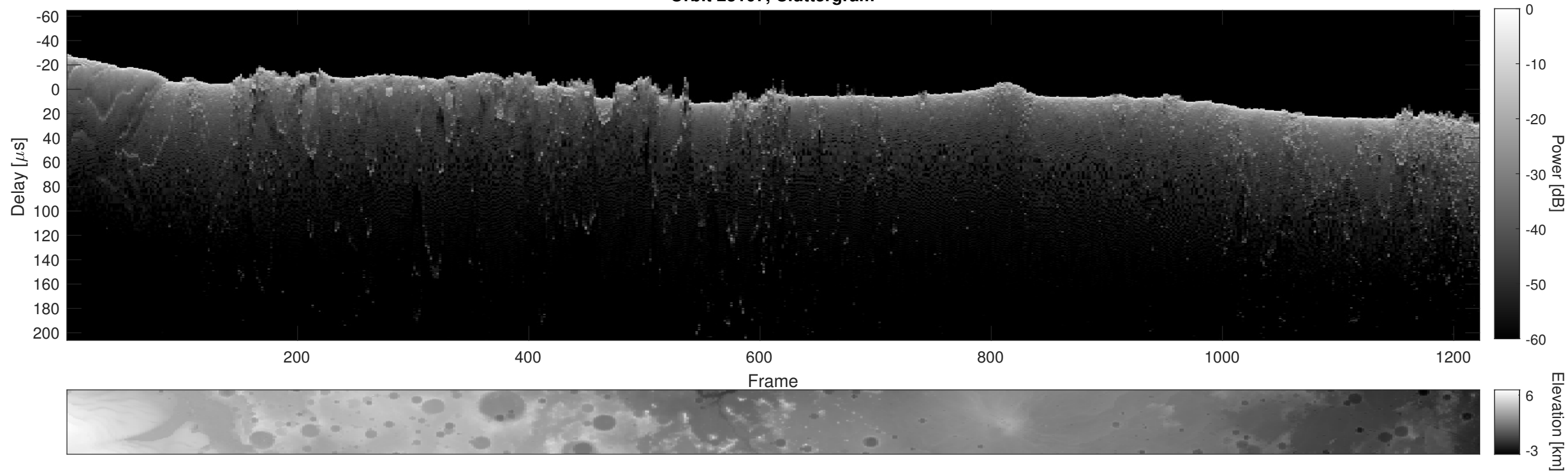
Orbit 23107, Cluttergram
