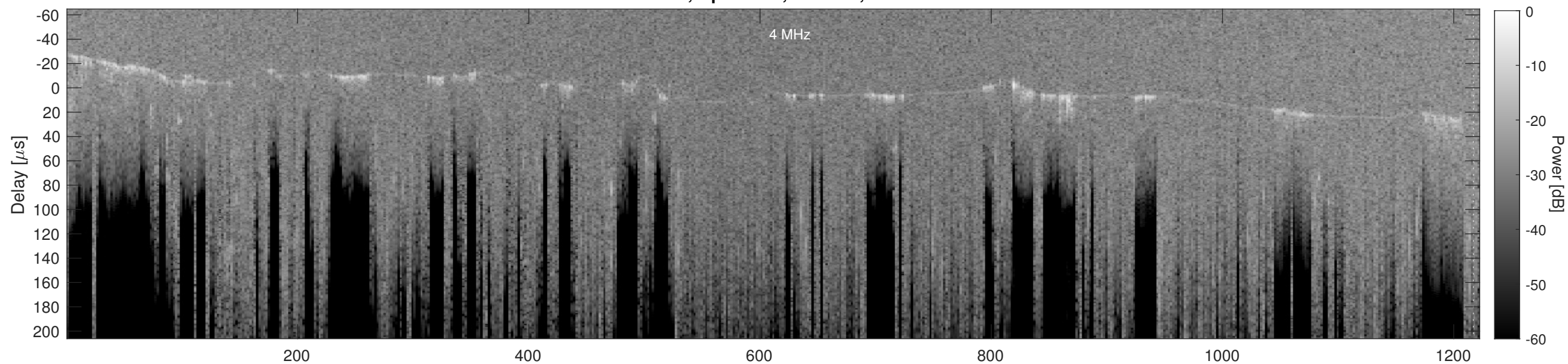
Orbit 23107, Cluttergram
