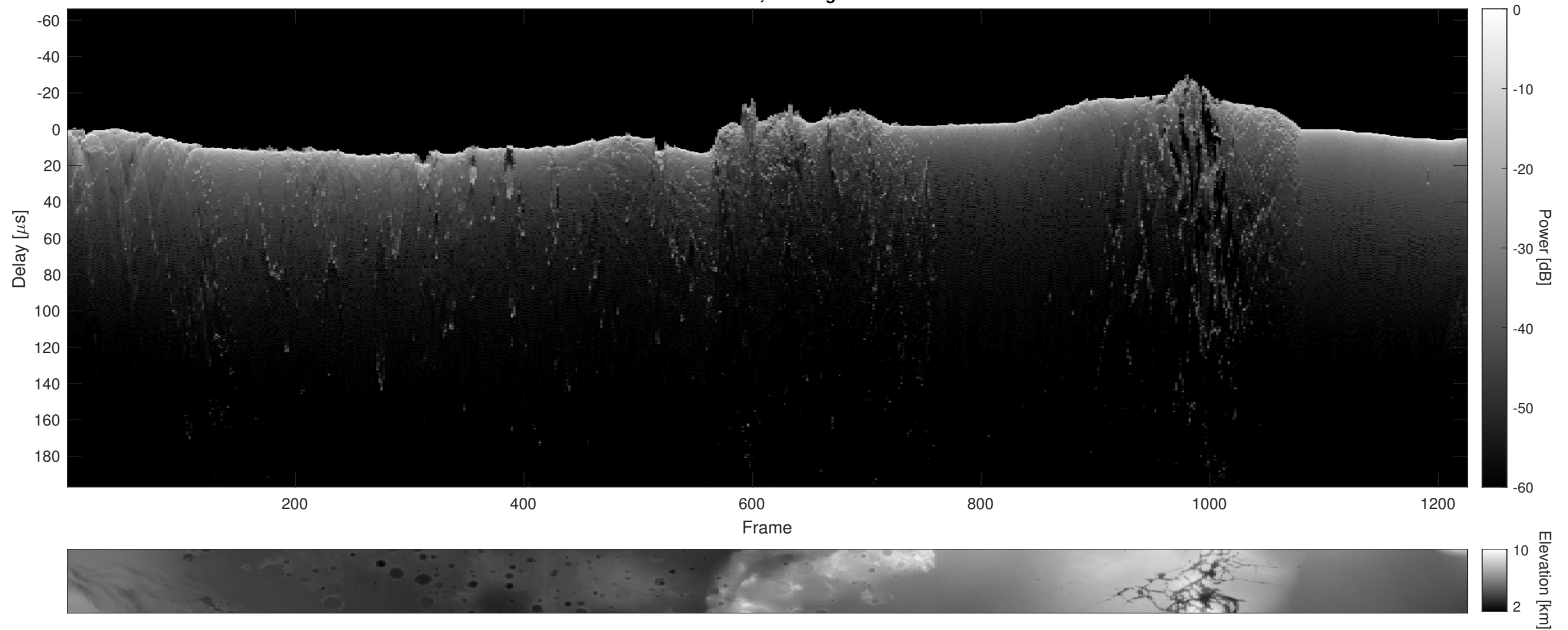
Orbit 23109, Cluttergram
