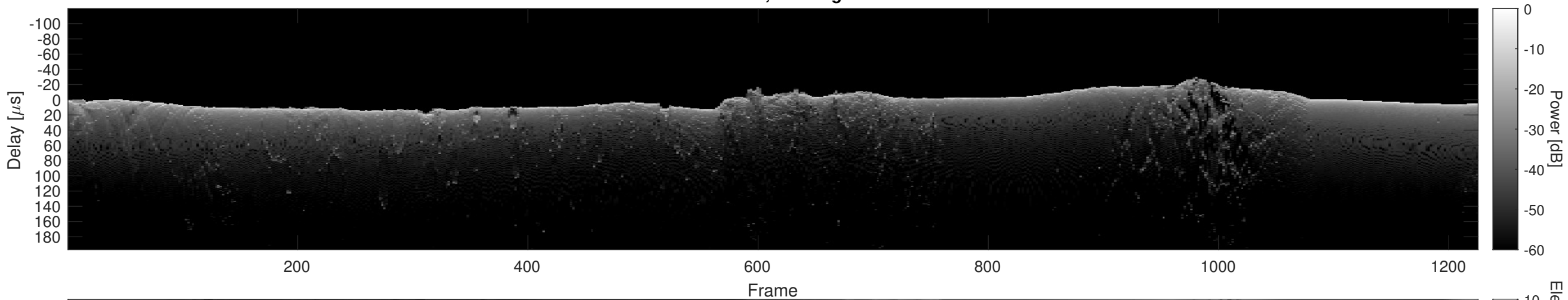
Orbit 23109, Cluttergram
