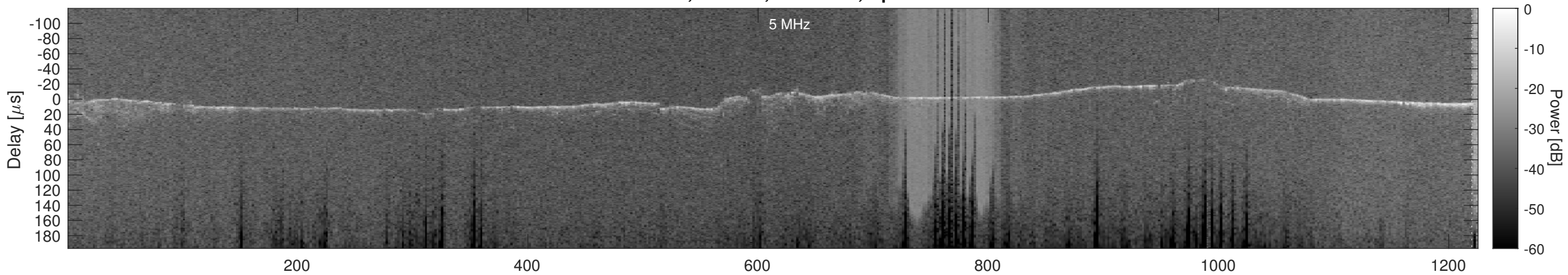
Orbit 23109, Cluttergram
