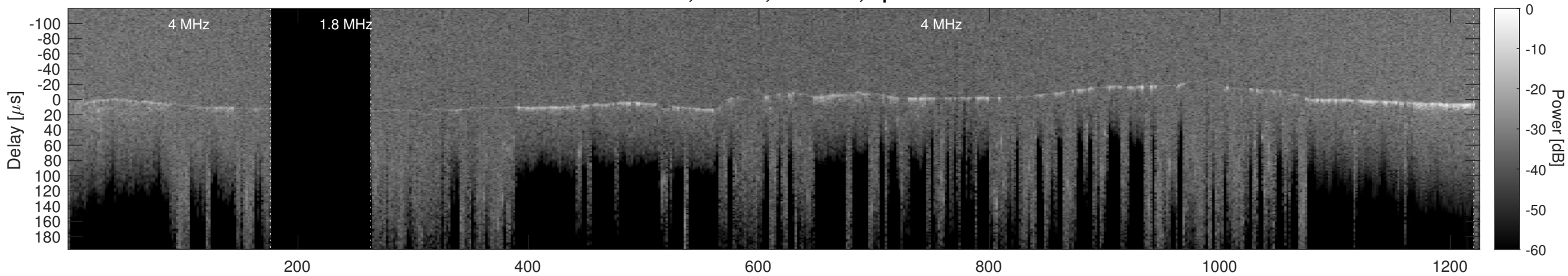
Orbit 23109, Cluttergram
