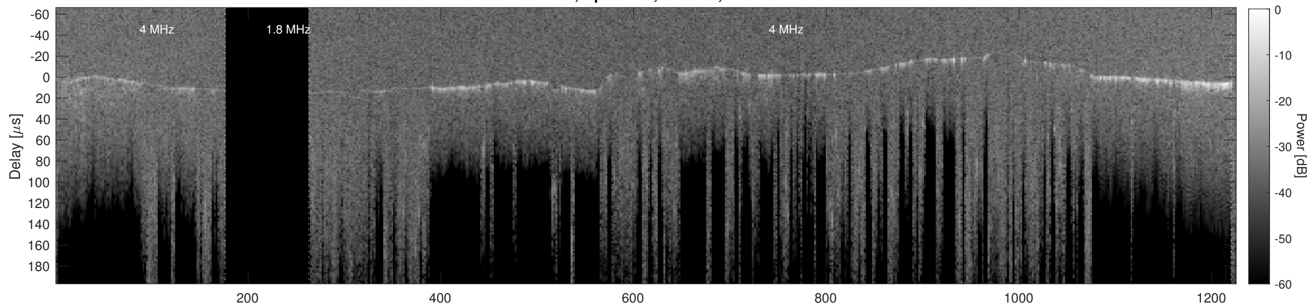
Orbit 23109, Cluttergram
