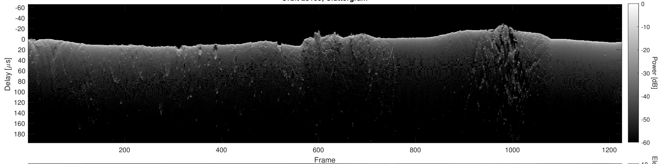
Orbit 23109, Cluttergram
