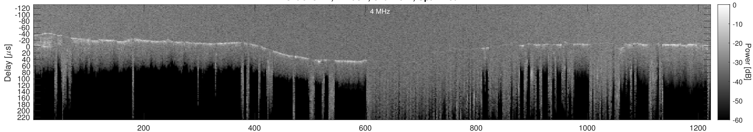
Orbit 23111, Cluttergram
