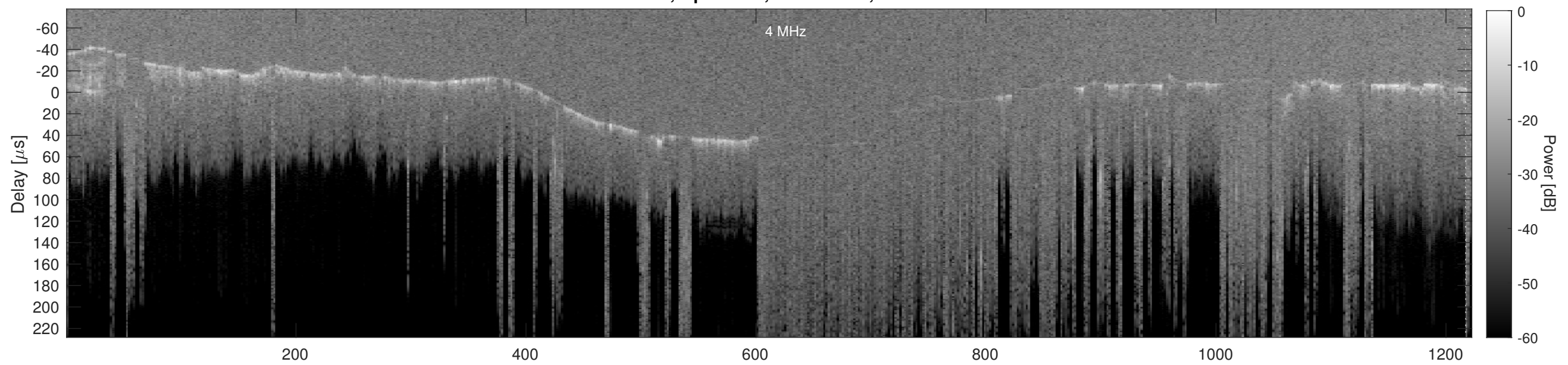
Orbit 23111, Cluttergram
