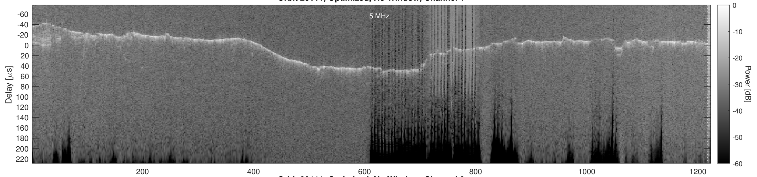
Orbit 23111, Optimized, No Window, Channel 2
