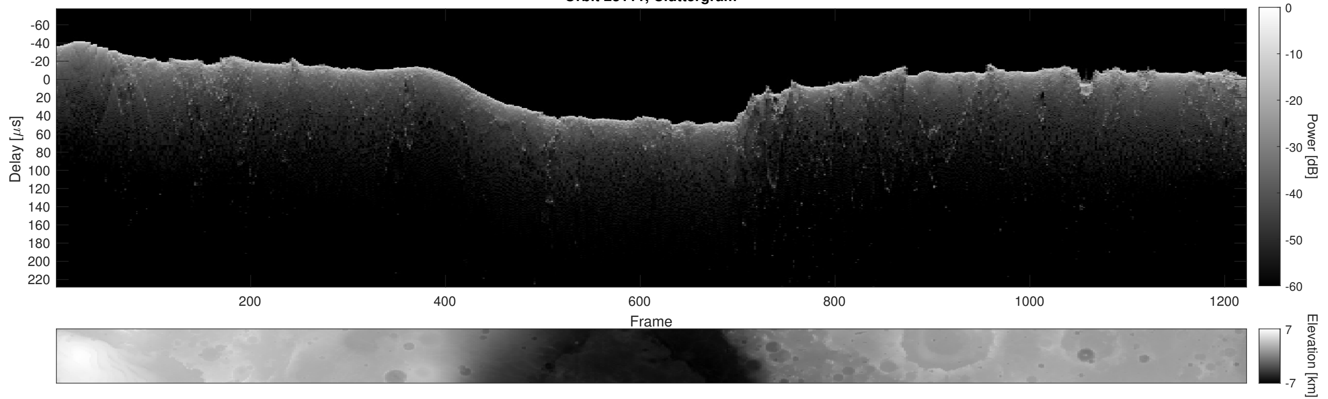
Orbit 23111, Cluttergram
