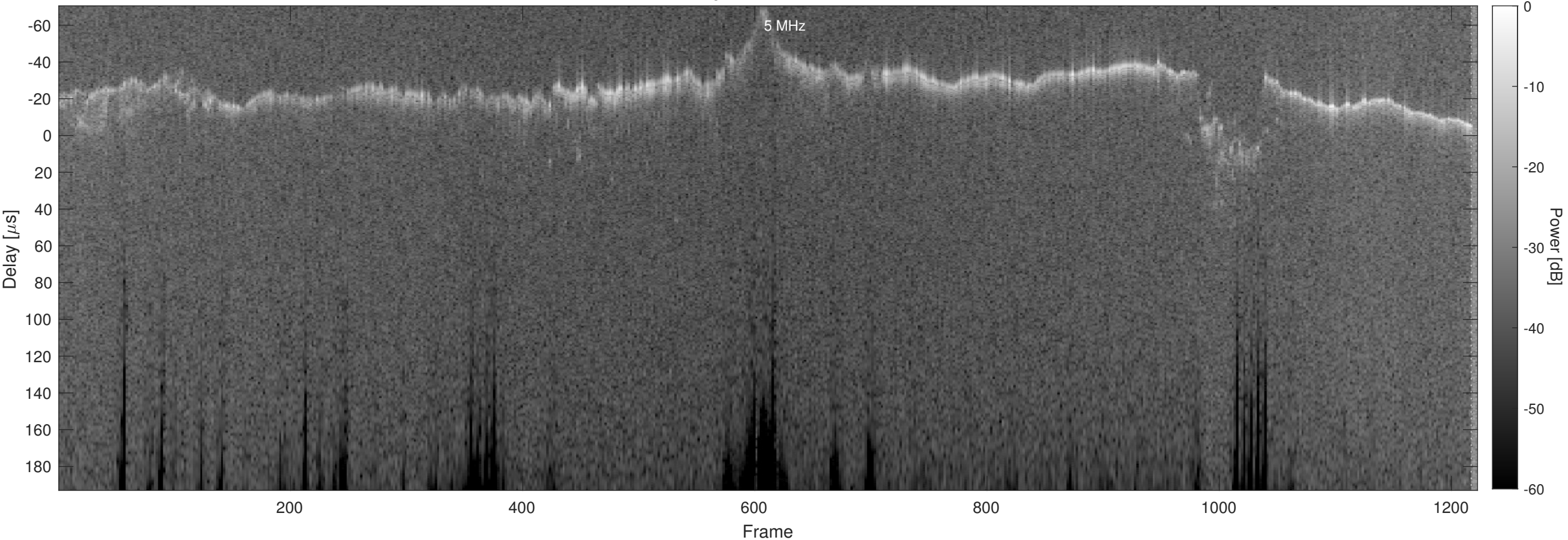
Orbit 23116, Chapman, No Window, Channel 2
