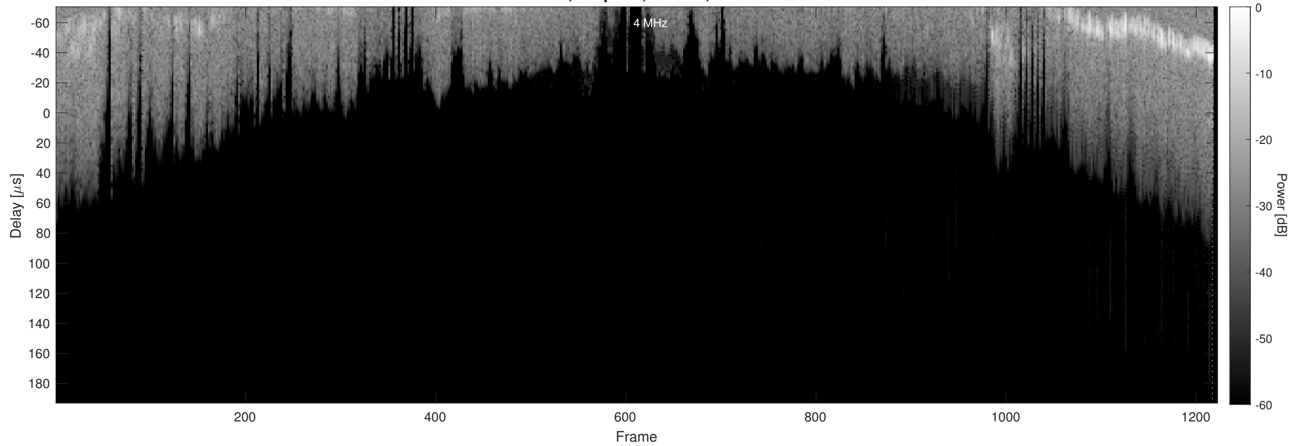
Orbit 23116, Chapman, Window, Channel 2
