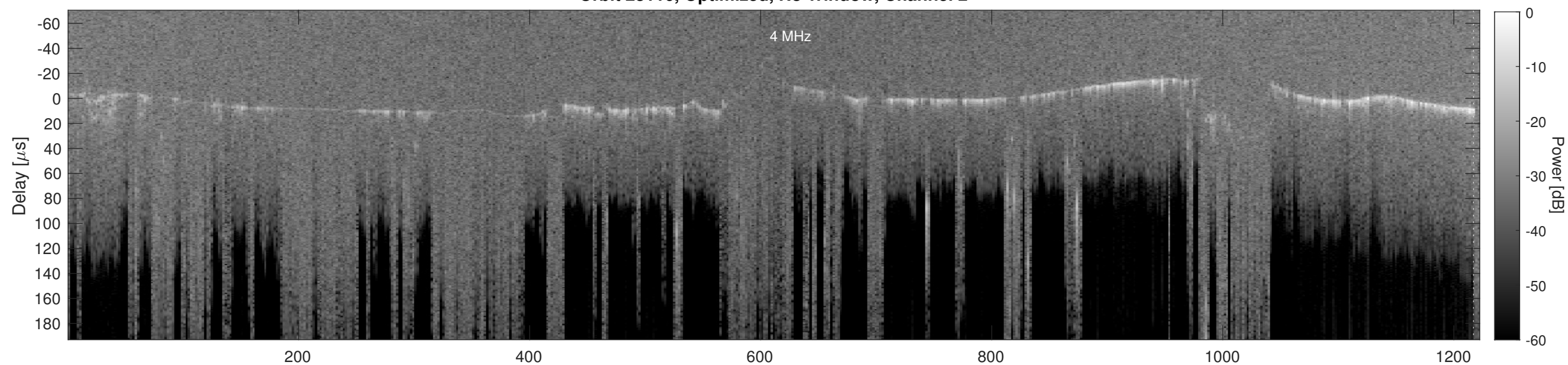
Orbit 23116, Cluttergram
