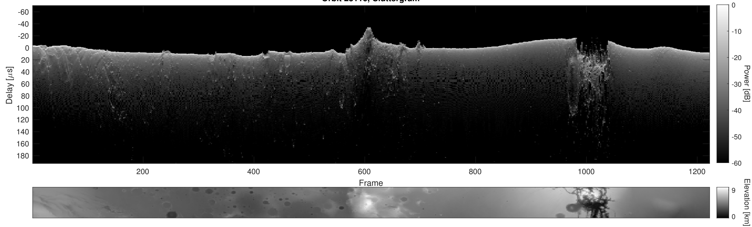
Orbit 23116, Cluttergram
