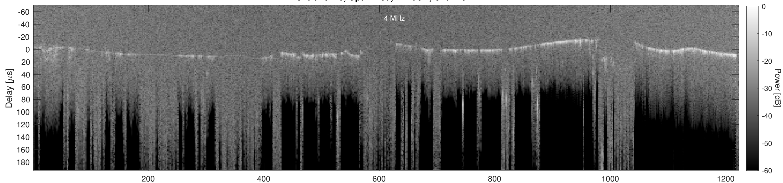
Orbit 23116, Cluttergram
