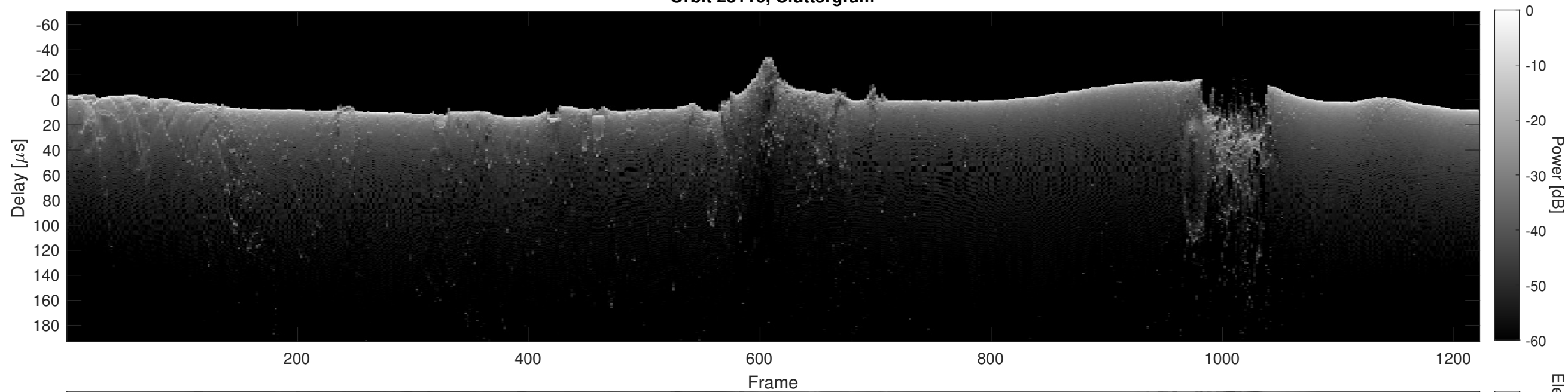
Orbit 23116, Cluttergram
