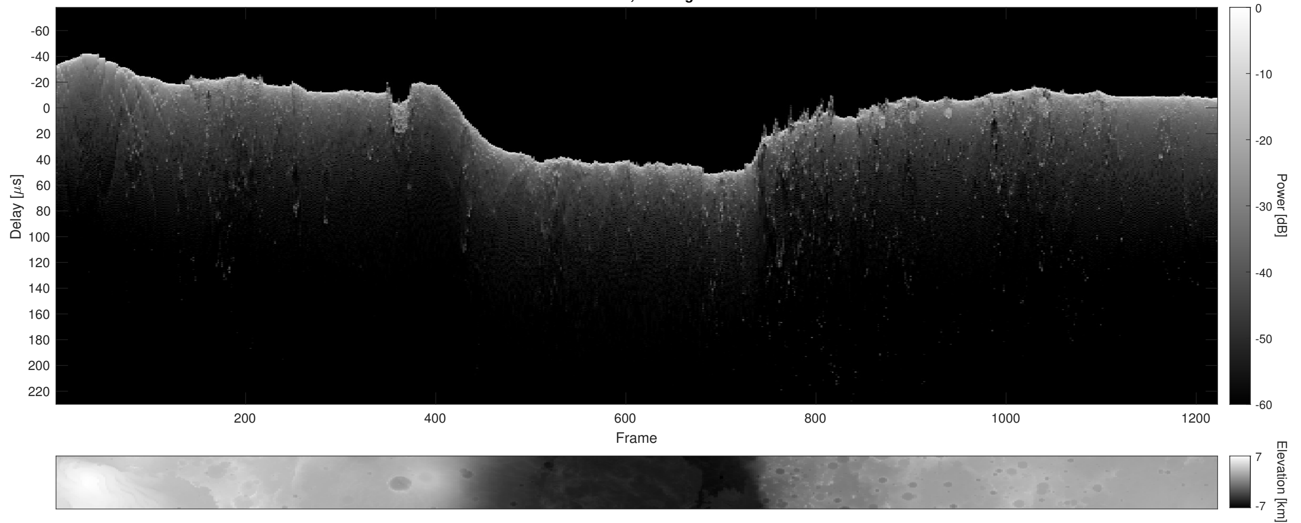
Orbit 23118, Cluttergram
