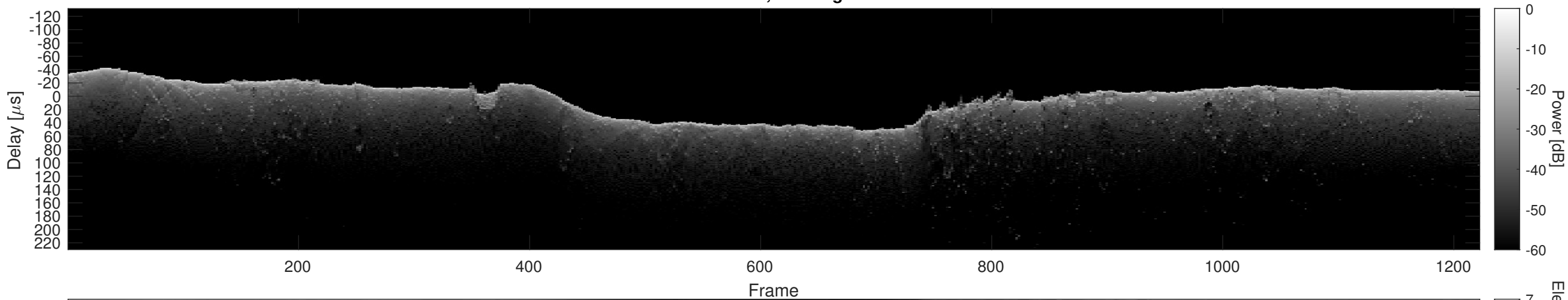
Orbit 23118, Cluttergram
