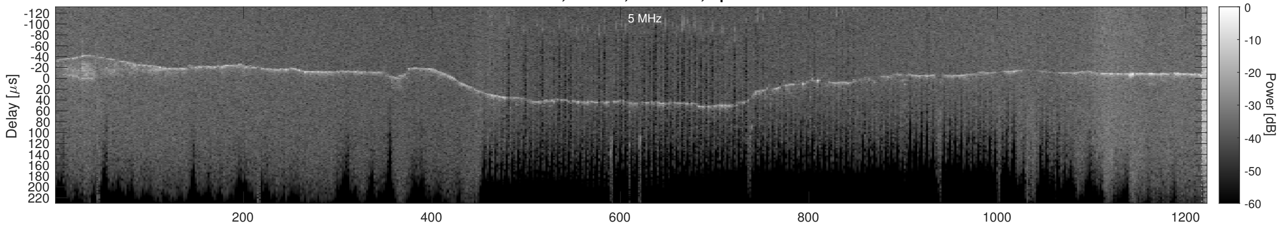
Orbit 23118, Cluttergram
