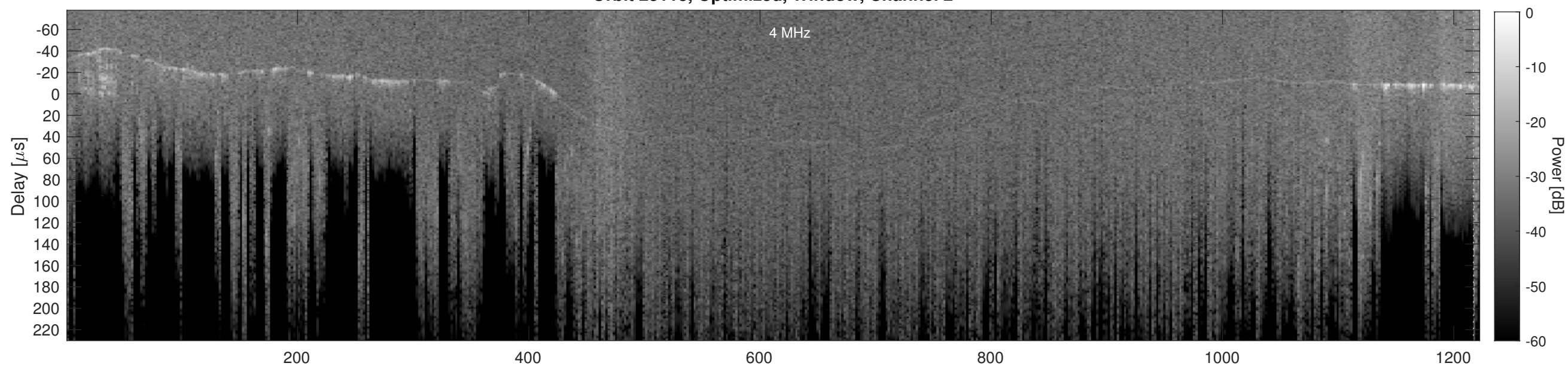
Orbit 23118, Cluttergram
