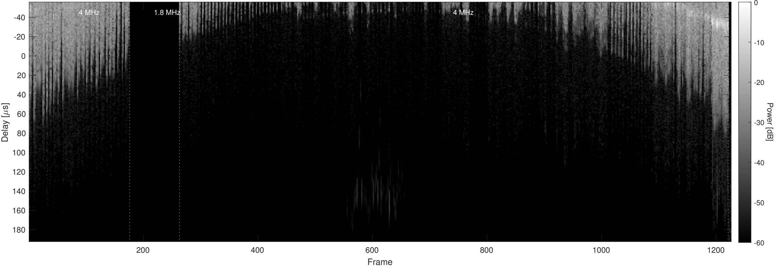
Orbit 23123, Chapman, No Window, Channel 2
