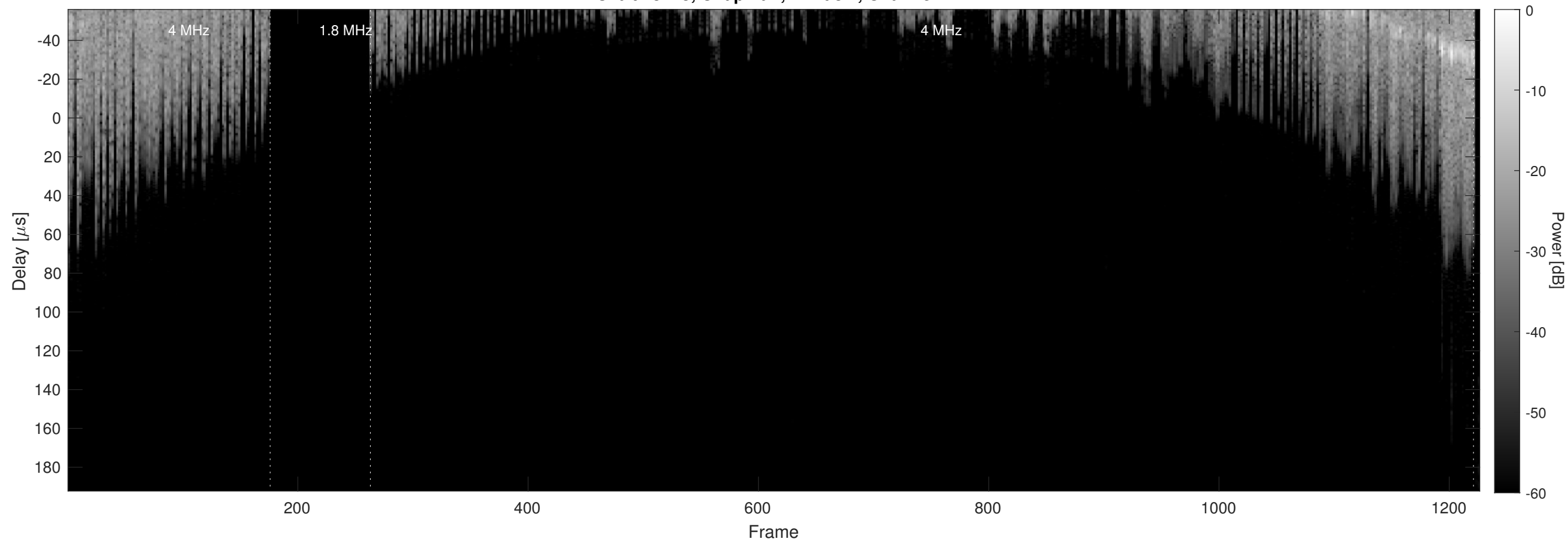
Orbit 23123, Chapman, Window, Channel 2
