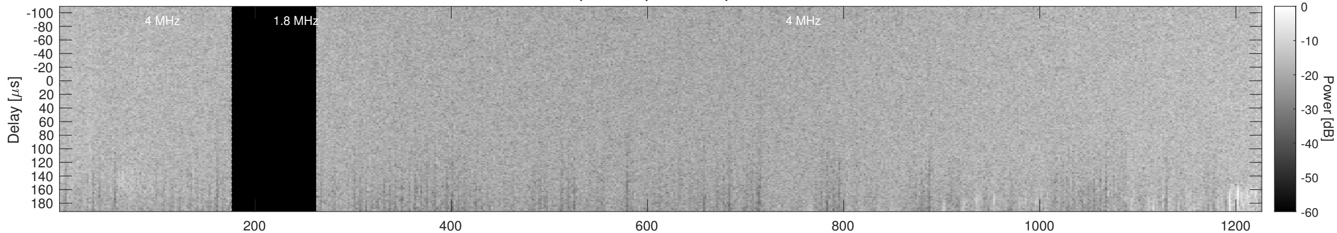
Orbit 23123, Window, Channel 2, Chapman
