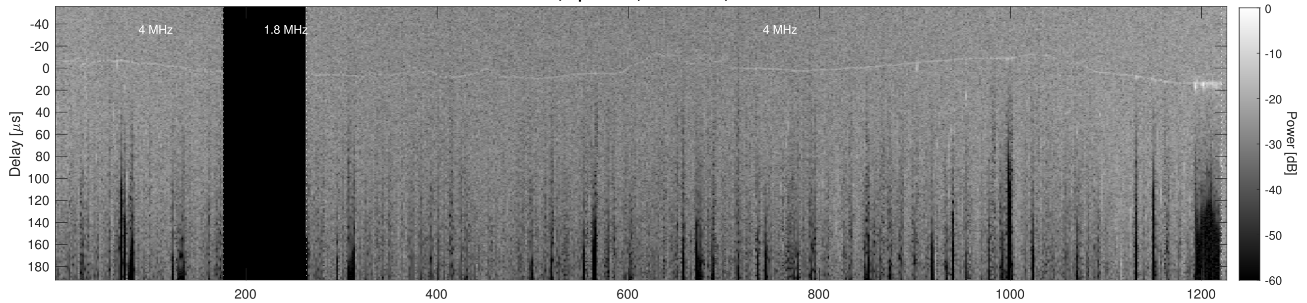
Orbit 23123, Cluttergram
