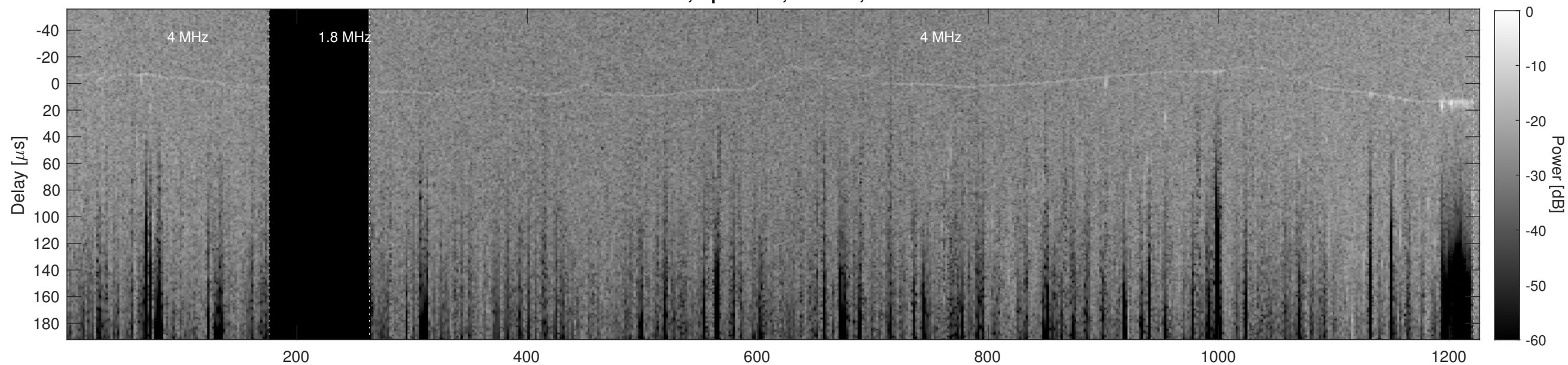
Orbit 23123, Cluttergram
