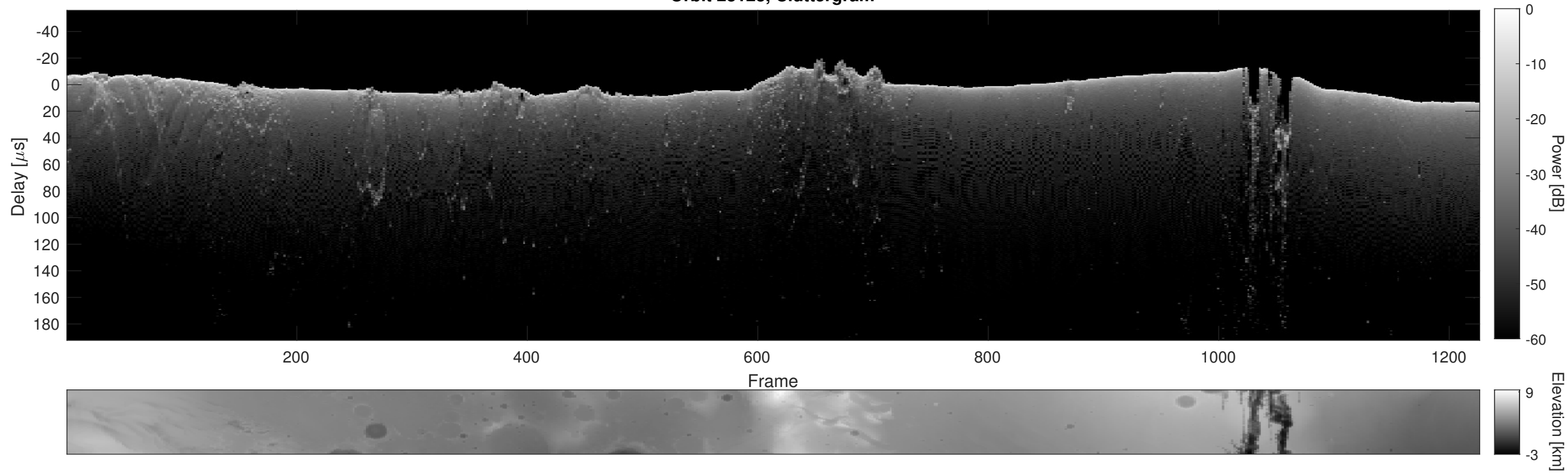
Orbit 23123, Cluttergram
