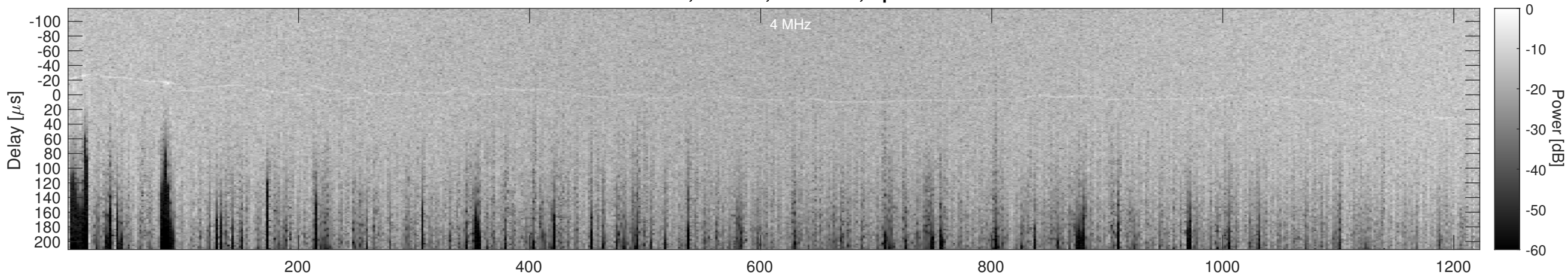
Orbit 23128, Cluttergram
