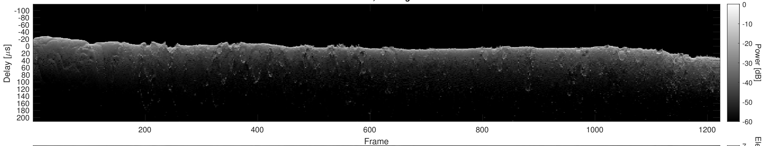
Orbit 23128, Cluttergram
