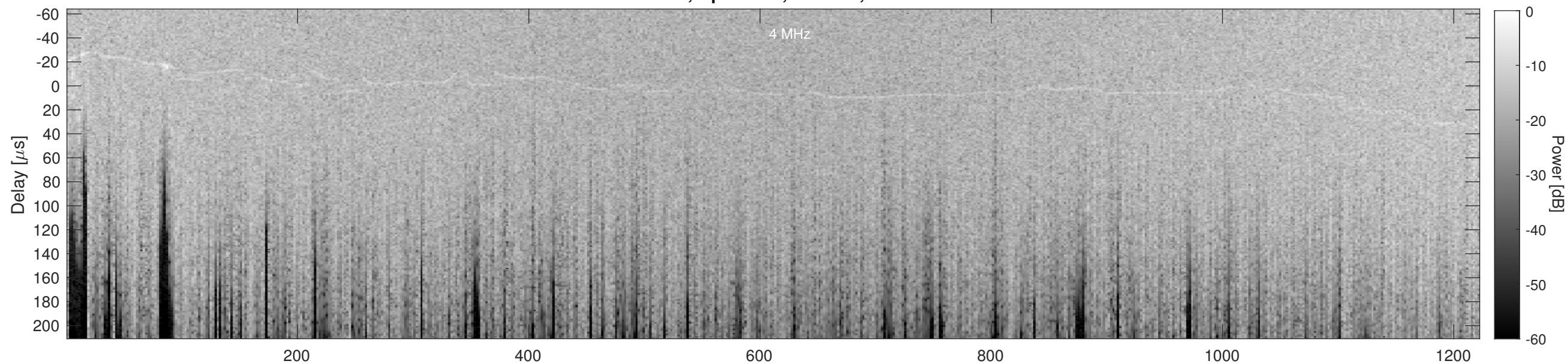
Orbit 23128, Cluttergram
