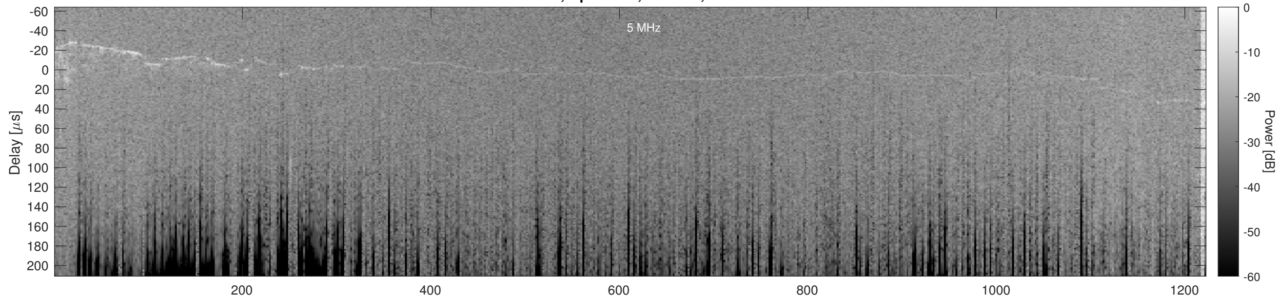
Orbit 23128, Optimized, Window, Channel 2
