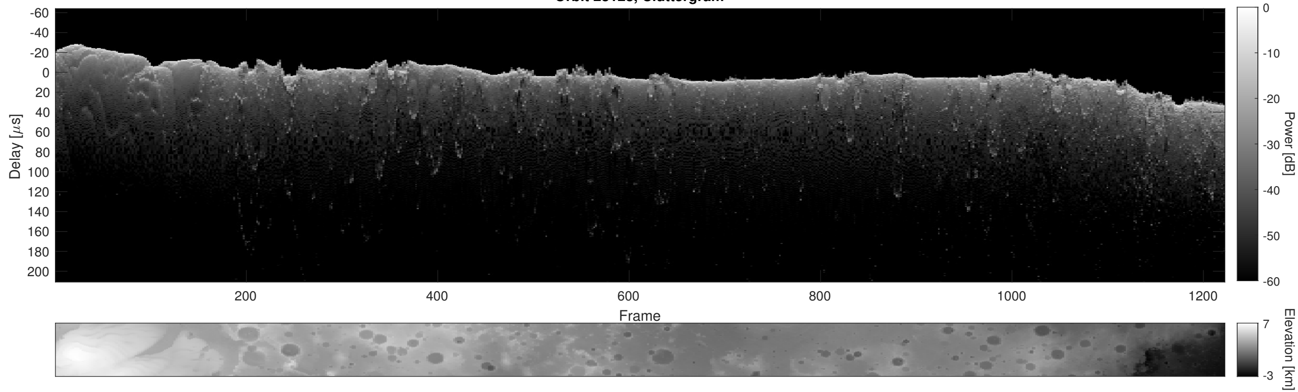
Orbit 23128, Cluttergram
