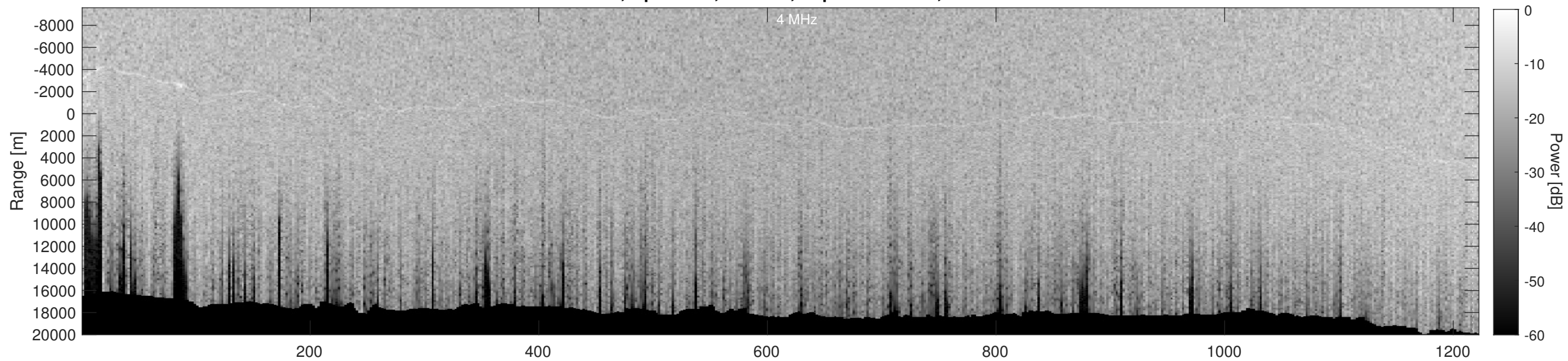
Orbit 23128, Depth-Corrected Cluttergram
