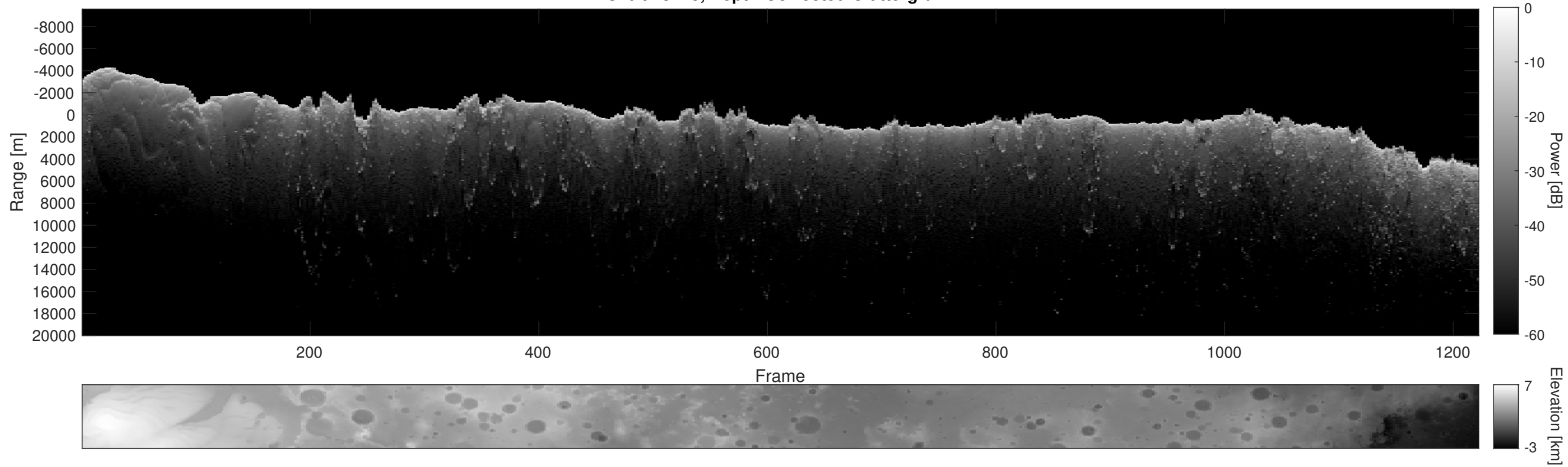
Orbit 23128, Depth-Corrected Cluttergram
