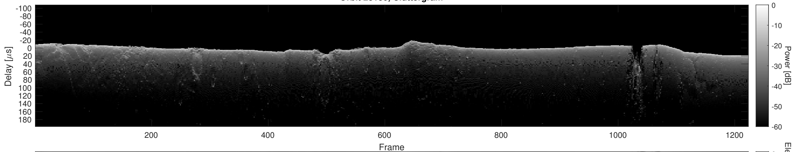
Orbit 23130, Cluttergram
