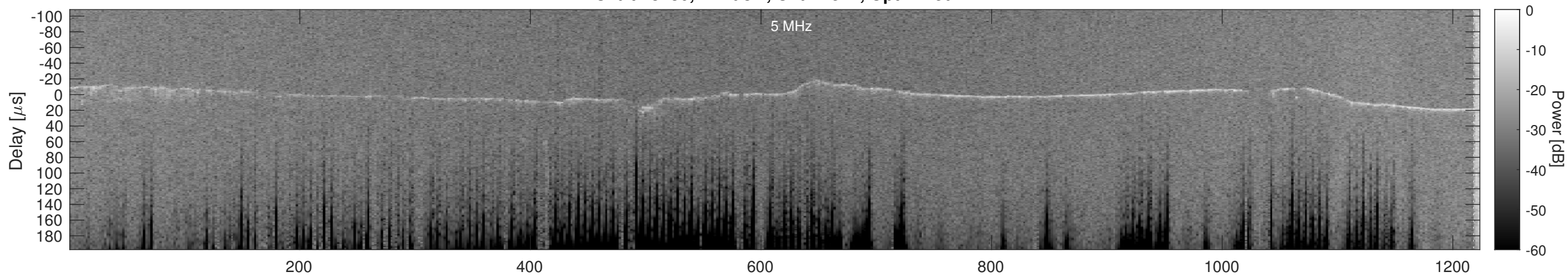
Orbit 23130, Cluttergram
