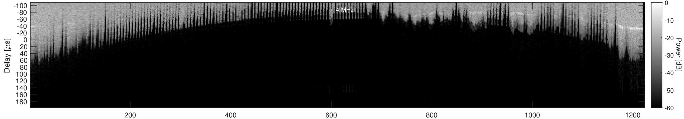
Orbit 23130, Window, Channel 2, Optimized
