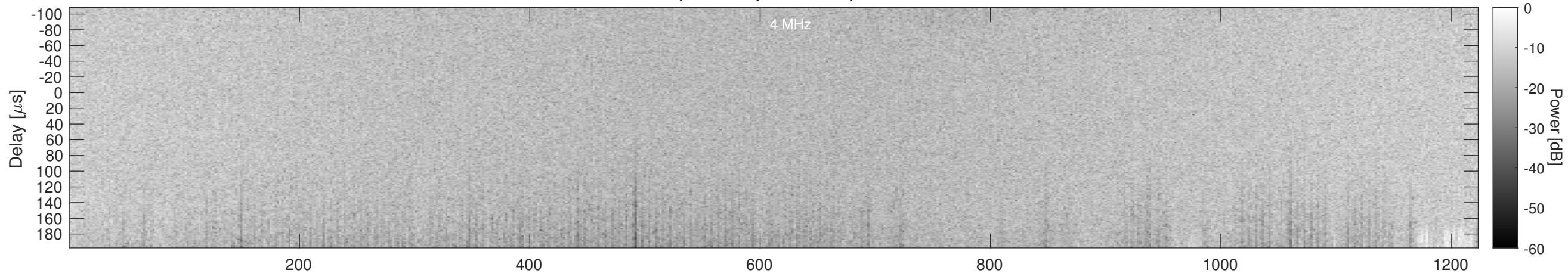
Orbit 23130, Window, Channel 2, Chapman
