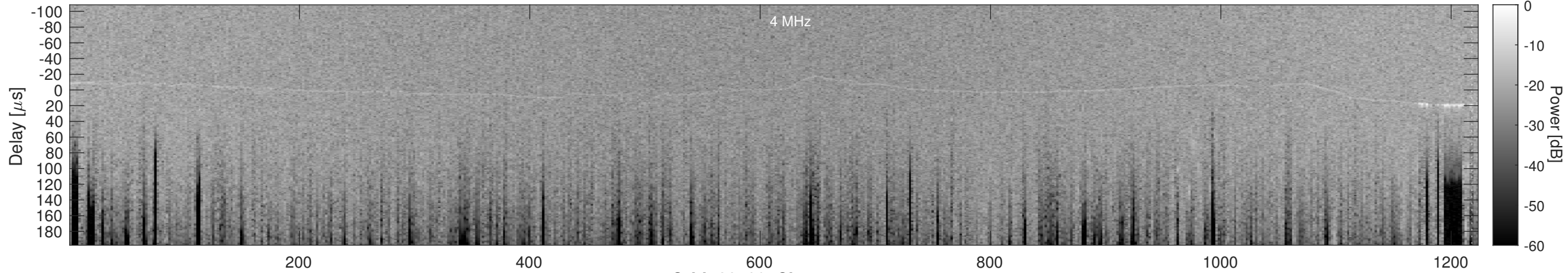
Orbit 23130, Cluttergram
