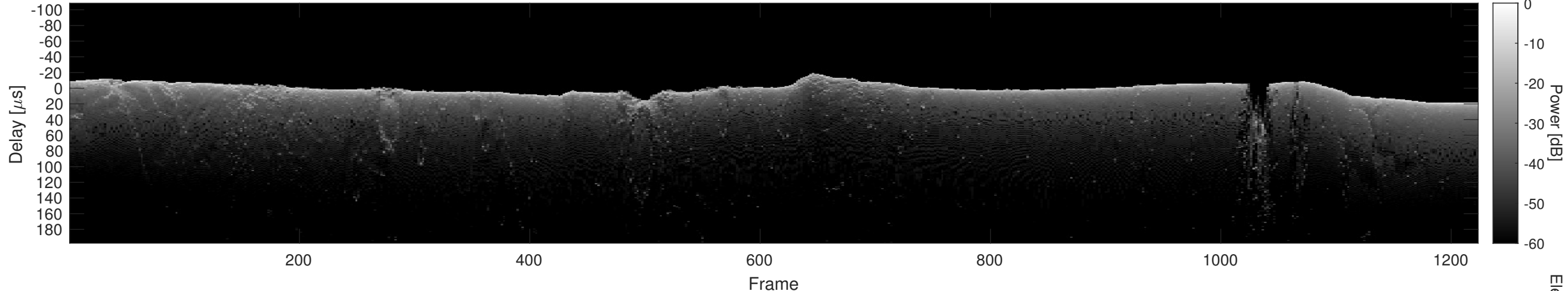
Orbit 23130, Cluttergram
