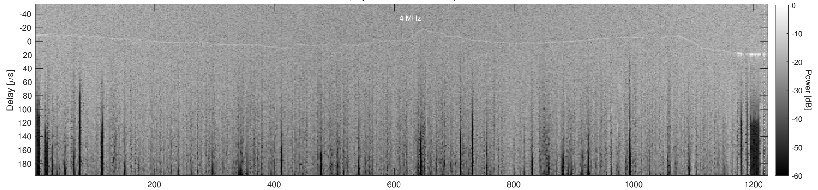
Orbit 23130, Cluttergram
